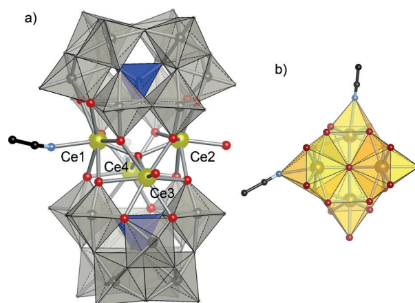
Figure 1. a, b) Polyhedral and ball-and-stick representation of the anionic component of CePOM (side view; a) and the tetranuclear Ce^{III} core in CePOM (top view; b). Carbon black, cerium yellow, nitrogen light blue, oxygen red, silicon blue, tungsten gray.
